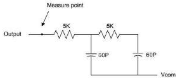
Output load condition
