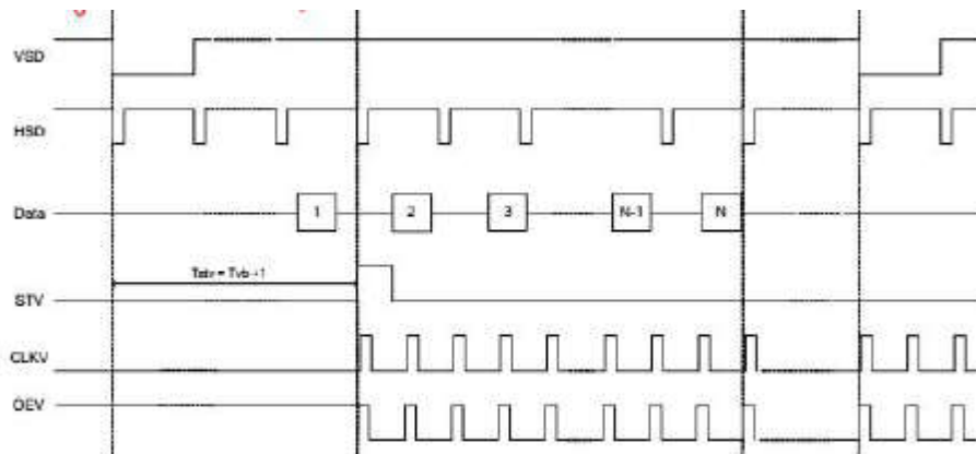
Vertical Timing Diagram HV
